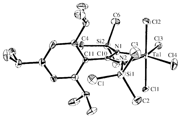
Fig. 1 Molecular structure of one of the two crystallographically independent molecules of [\text{Ta}\{(2,4,6\text{-tri-}^i\text{Pr})\text{C}_6\text{H}_2\text{C}(\text{NSiMe}_3)_2\}\text{Cl}_4] ( 2 ). Hydrogen atoms omitted for clarity.
