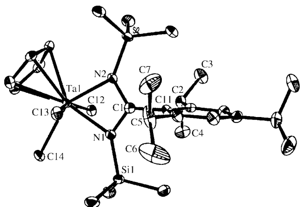
Fig. 4 Molecular structure of [\text{Ta}\{(2,4,6\text{-tri-}^i\text{Pr})\text{C}_6\text{H}_2\text{C}(\text{NSiMe}_3)_2\}(\eta\text{-C}_5\text{H}_5)\text{Cl}_3] ( 10 ). Hydrogen atoms omitted for clarity.
