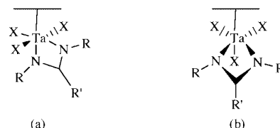
Fig. 6 The two structure types observed for compounds of the general formula [\text{Ta}\{\text{R}'\text{C}(\text{NR})_2\}\text{Cp}'\text{X}_3] ( \text{Cp}' = \text{Cp}^* or \text{Cp} , \text{R}' = \text{Me} , p\text{-MeO-C}_6\text{H}_4 or 2,4,6\text{-}^i\text{Pr}_3\text{-C}_6\text{H}_2 ; \text{R} = ^i\text{Pr} or \text{SiMe}_3 ; \text{X} = \text{F} , \text{Cl} or \text{Me} ).
